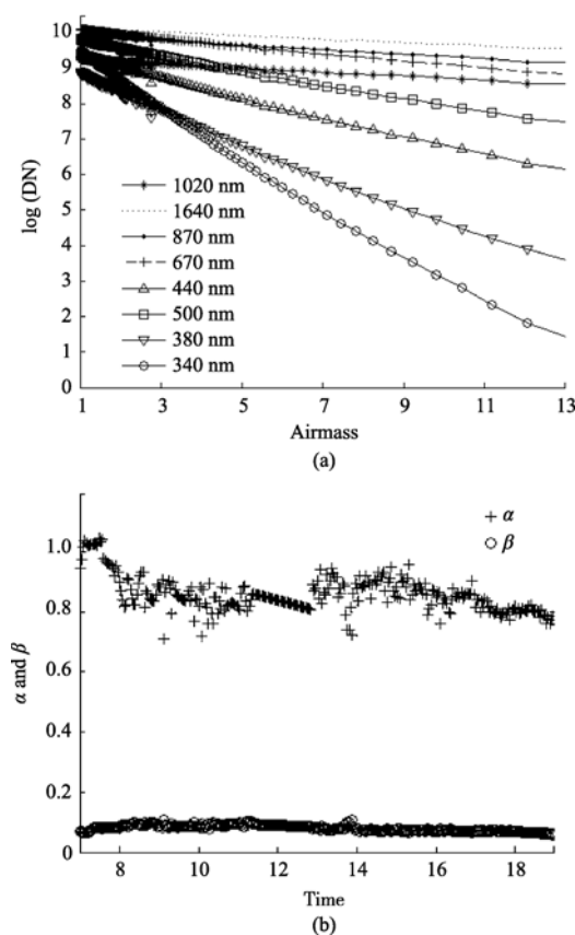
Fig. 4 Optical properties of atmospheric aerosol on June 1, 2007 (a) Lanley-plot result of CE318's data; (b) Ångström parameters
